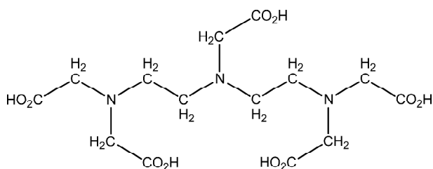
Figure 3. Chemical structure of diethylenetriaminepentaacetic acid (Hdtpa).
